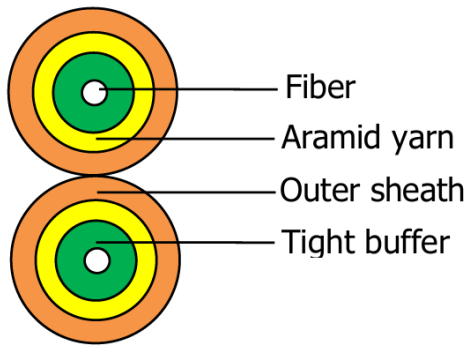
Structural Diagram
